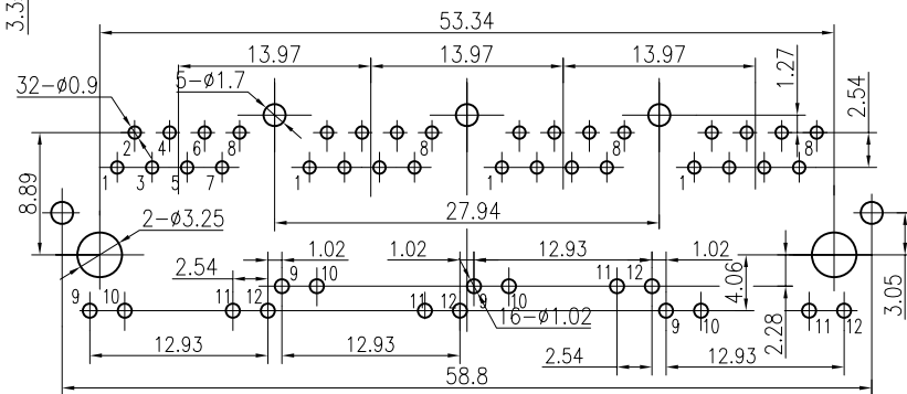
PCB BOARD LAYOUT
