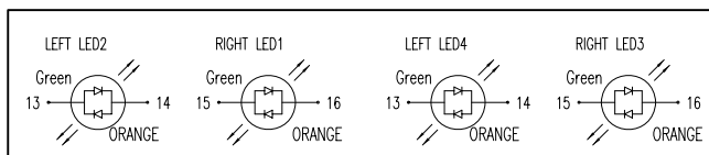
LED Specification
