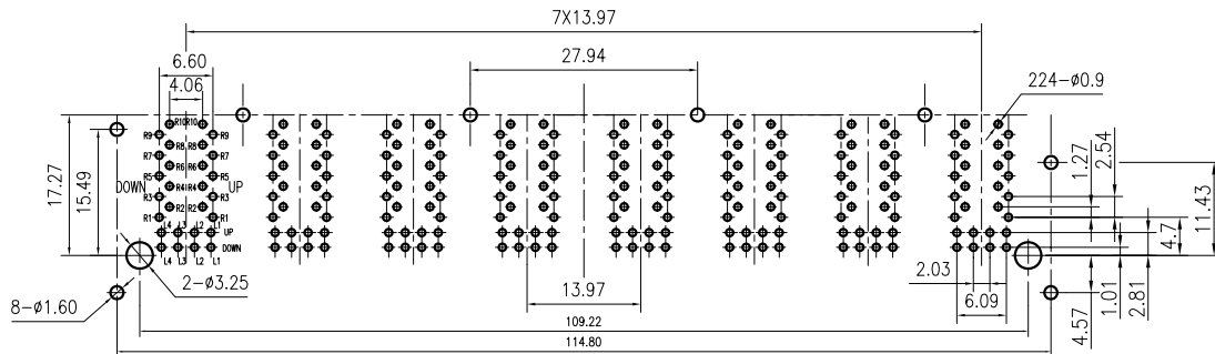
PCB BOARD LAYOUT
