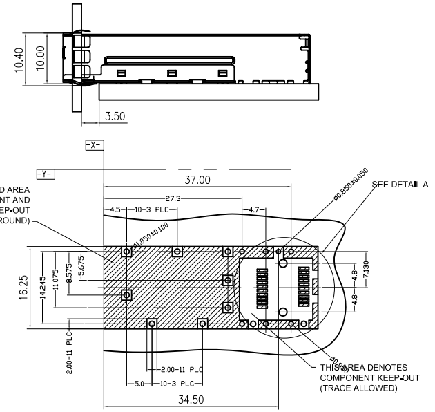
PCB LAYOUT THICKNESS=3.0mm (TOP VIEW)
