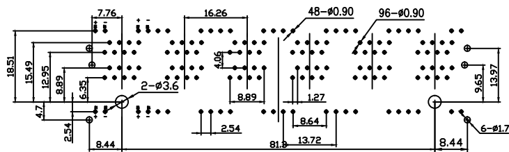
PCB LAYOUT TOLERANCE:±0.05
